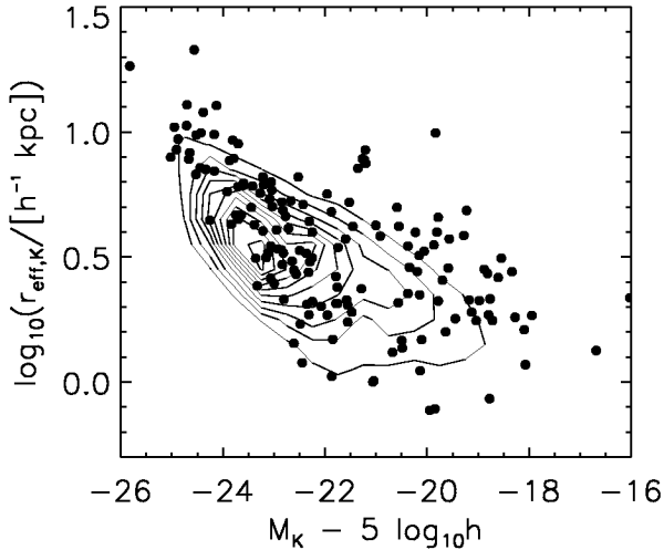
FIG. 1.— K -band magnitude and half-light radius for the 6573 late-type SDSS+2MASS galaxies in our sample ( contours ) and for the 156 galaxy comparison sample of Bell & de Jong (2000; filled circles ).
