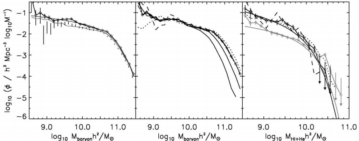
FIG. 2.—Baryonic MF of galaxies. Left panel: Stellar MF of Cole et al. (2001; naked error bars ) corrected to our maximum disk IMF, the stellar MF derived using our SDSS g -band-selected sample ( solid gray line ), and the baryonic MF of galaxies, assuming the maximum disk IMF ( solid line with open circles and error bars , with a Schechter fit as the thin solid line). Middle panel: Different versions of the baryonic MF, illustrating the different sources of uncertainty. The solid line with open circles again is the baryonic MF defined using the default gas mass estimation technique, the dashed line shows the effect of choosing the nearest galaxy on the half-light radius–luminosity plane for estimating the gas mass, the dotted line shows the effect of allowing SDSS+2MASS early-type galaxies to also have gas, and the two solid lines are the effect of choosing a Kennicutt or Kroupa IMF ( upper line ) or an M/L ratio consistent with a Bottema disk ( lowest line ). Right panel: We test the gas mass estimation method by comparing the H I and H 2 MFs predicted using this method with observations. The solid line with open circles and error bars denotes the match of SDSS+2MASS spiral galaxies with randomly selected nearby galaxies, and the dotted and dashed lines are as in the middle panel. The solid black curve is the blind H I MF of Rosenberg & Schneider (2002). The H 2 galaxy MF is shown as the gray line with open circles and error bars, and the Schechter fit to the first observational estimate of the H 2 MF (from Keres et al. 2003) is shown as the solid gray line.
